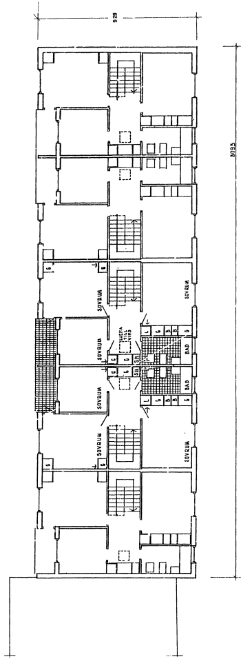
PLAN 1 TR.
